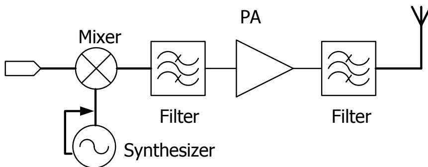
Figure 1 RFDK-TX Schematic Diagram
